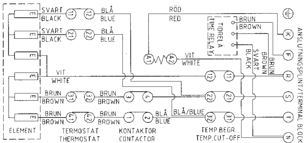
Wiring diagram
