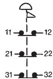
Wiring diagram
