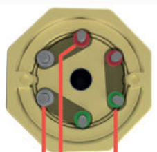
L1 L2 L3 Triangle connection
