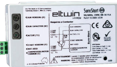
Standard Single-Phase Model
