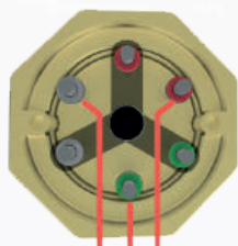
L1 L2 L3 Star connection
