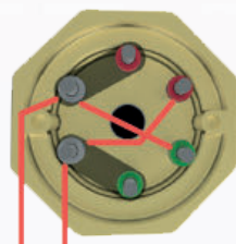
L1 L2 1-phase 3 elements
