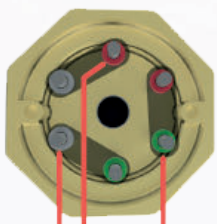
L1 L2 L3 Triangle connection
